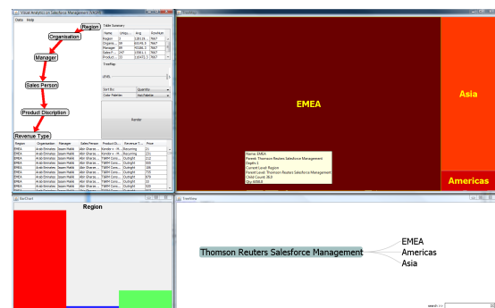
Figure 1: This image shows the general overview of our system. The two windows on the left are the control panels which summarize and manipulate the ontological hierarchy information. The two windows on the right are the coordinated views of treemap and DOI tree. They both form a structure-aware visualization for hierarchical data.
