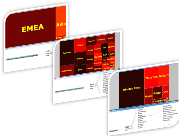
Figure 3: This image shows how the DOI tree can be coordinated with our squarified treemap.
