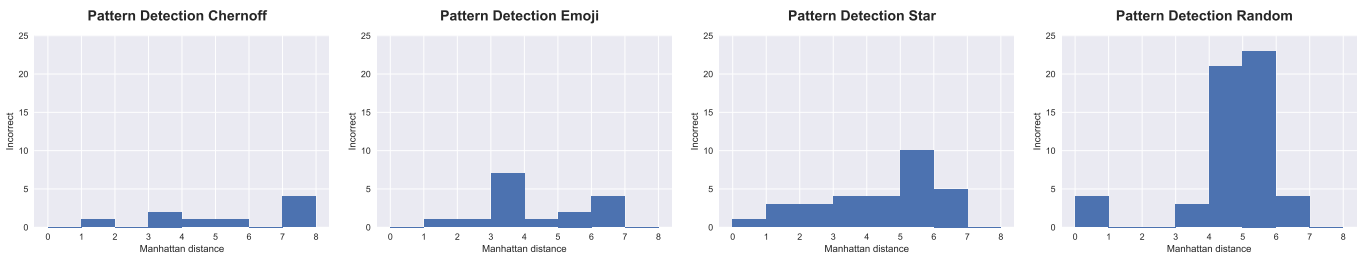
Figure 8: Manhattan distances of target versus answer for Task 3. Data shows the number of incorrect answers and distance from target.
