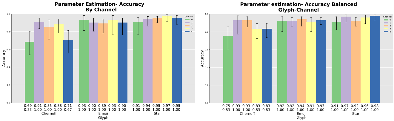
Figure 9: Analysis of accuracy results for Task 1 & 4 – Parameters Estimation (unbalanced vs. balanced). Results are broken down by channel for each visual encoding, (mean, median) values are indicated below each bar. Error bars show 95% confidence intervals.
