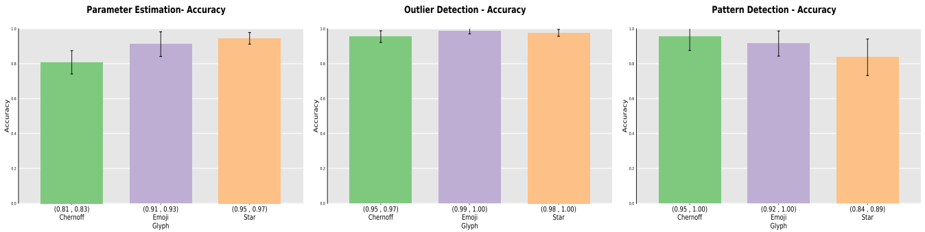
Figure 4: Analysis of accuracy results for Task 1, 2 & 3 respectively. Results shown for each visual encoding, (mean, median) values are indicated below each bar. Error bars show 95% confidence intervals.
