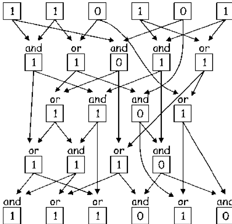
Fig. 3. A boolean circuit used as a one-way function for the coin-toss.
