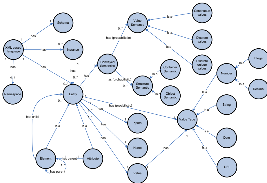
Figure 3 : The XML Entities Ontology
