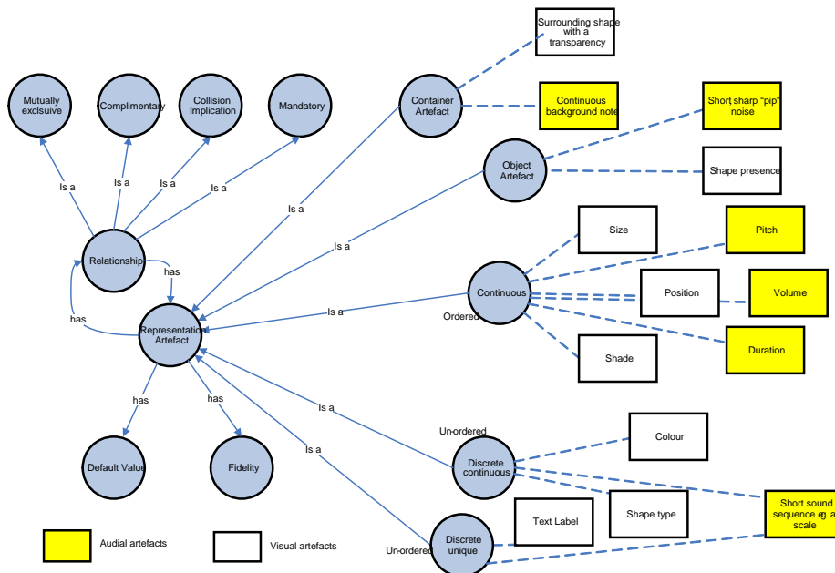
Figure 4 : The Representation Artefacts Ontology
